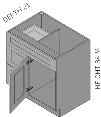
Shown as left side hinges. Drawers left.
