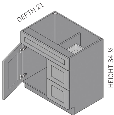
Shown as left side hinges. Drawers right.
